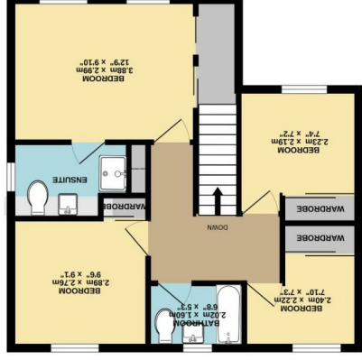
1ST FLOOR 48.6 sq.m. (523 sq.ft.) approx.
